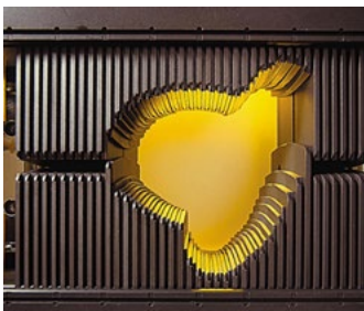
Multileaf collimator
